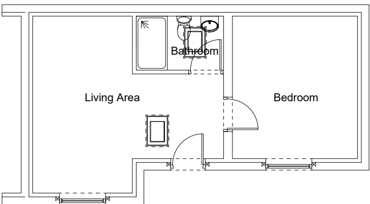
Proposed Layout
