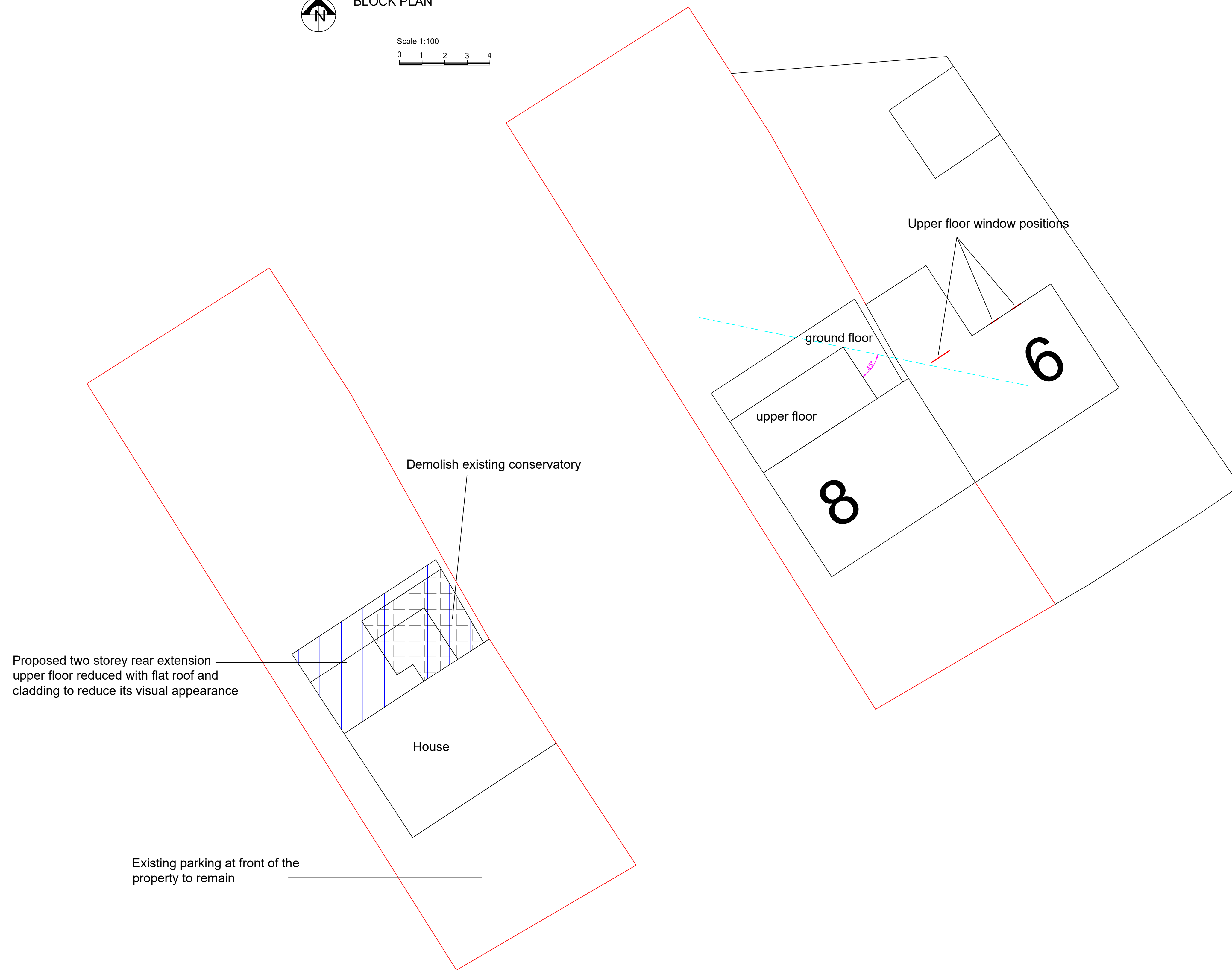
BLOCK PLAN
