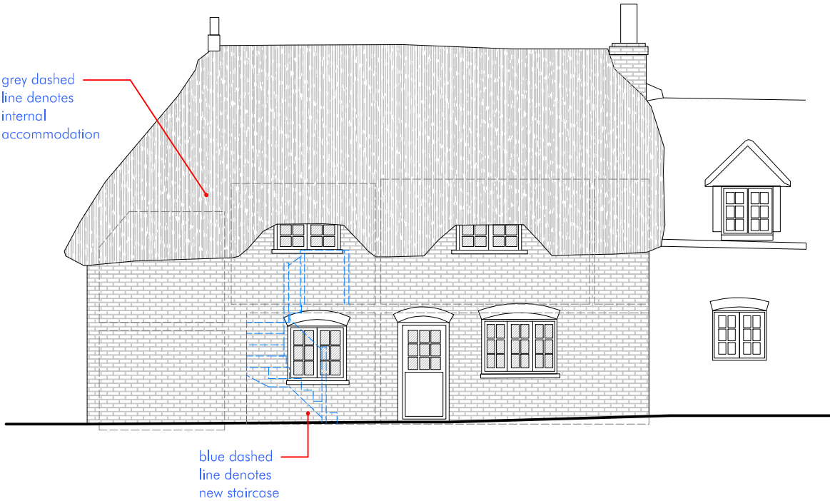
East Elevation
