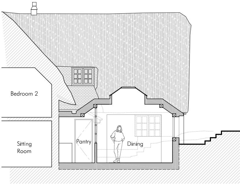
Section C-C
