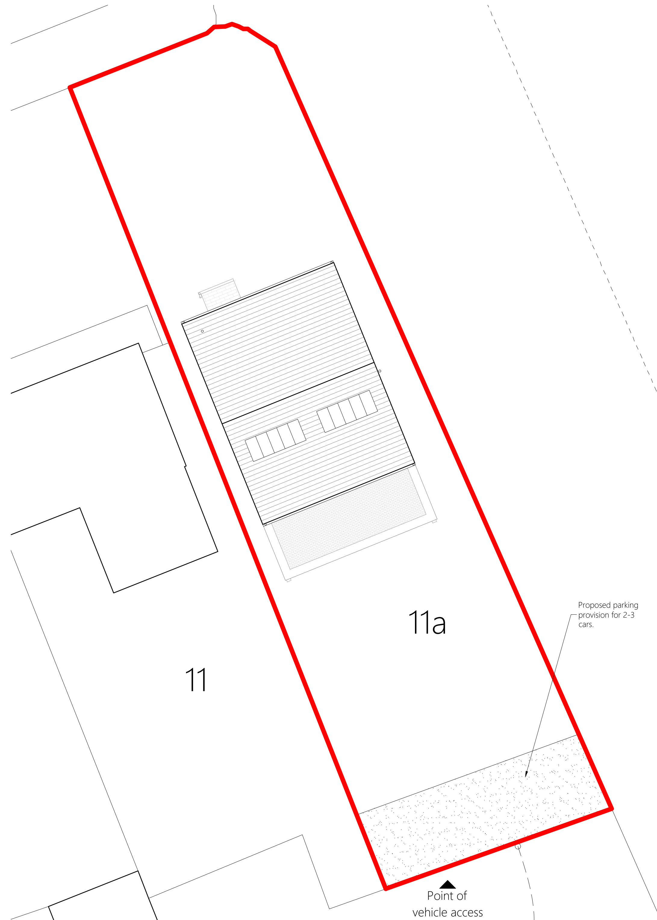
2 Plan Site Proposed arrangement 1:100 @ A1 200
