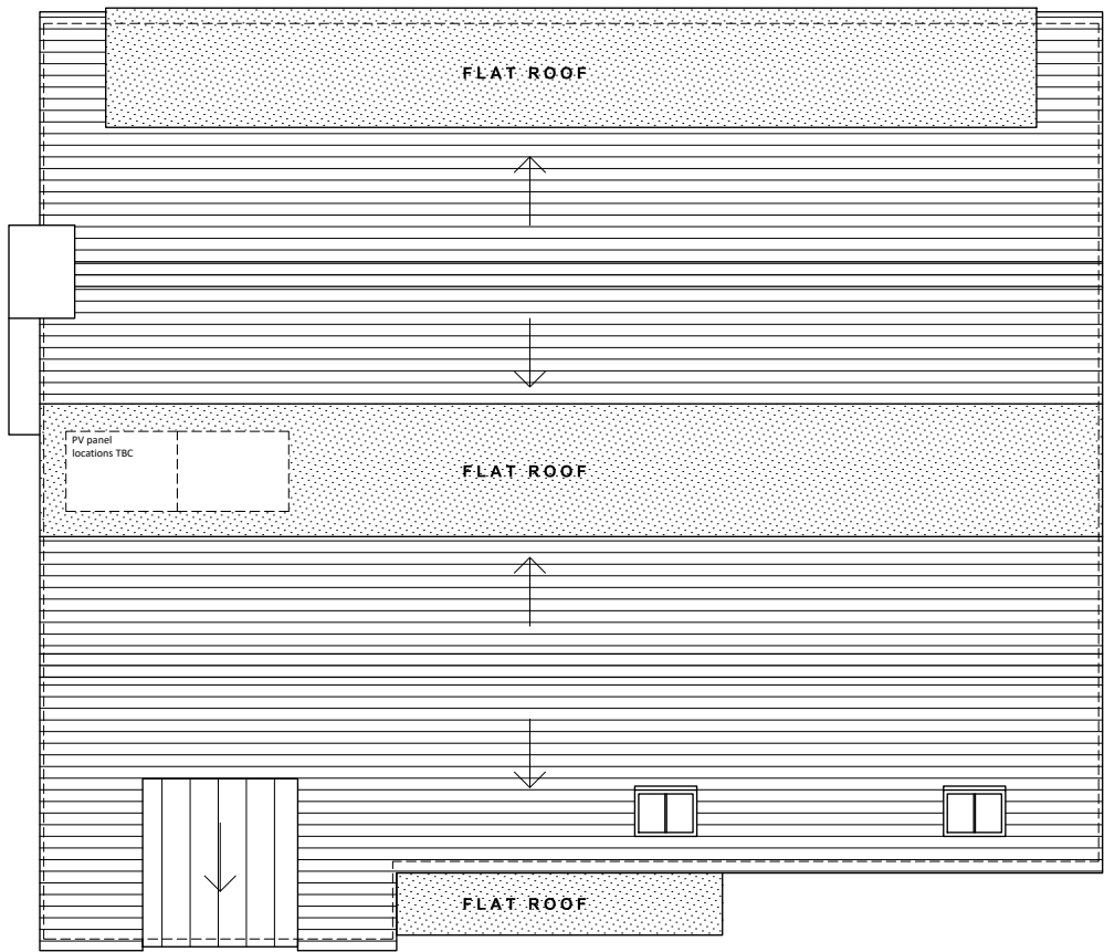
ROOF PLAN
