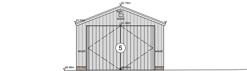
ELEVATION E GARAGE NORTH-WEST
