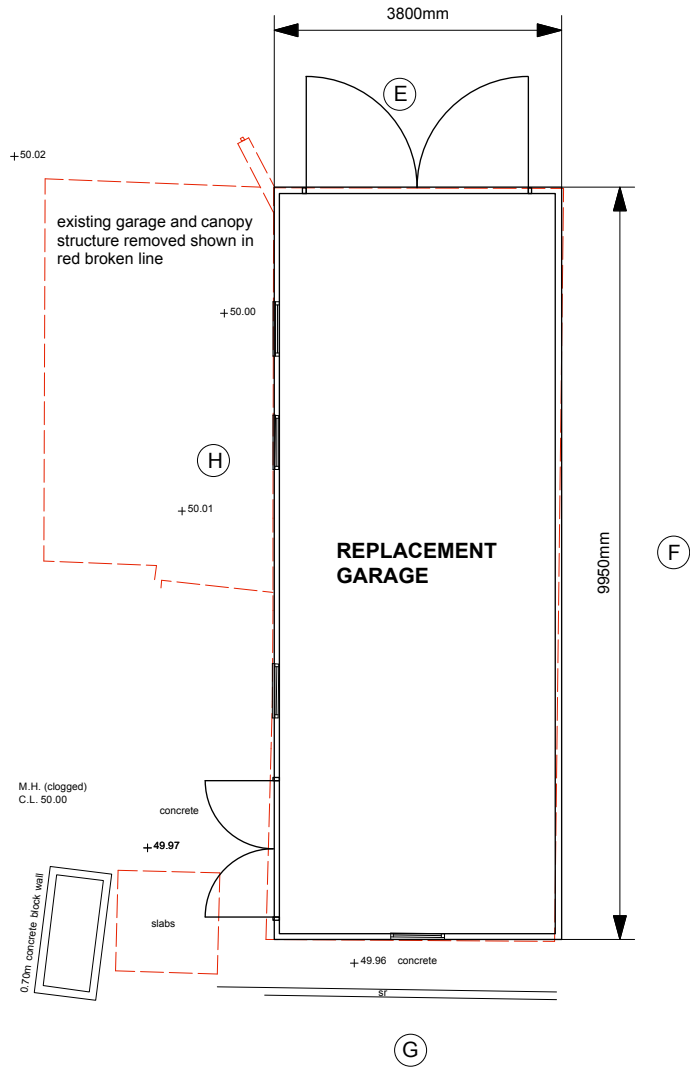
PROPOSED REPLACEMENT GARAGE PLAN
