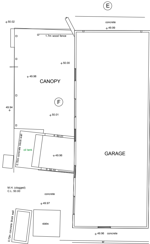
EXISTING GARAGE PLAN
