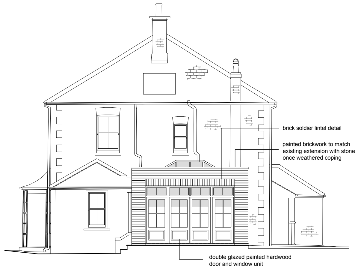
SOUTH EAST ELEVATION - PROPOSED
