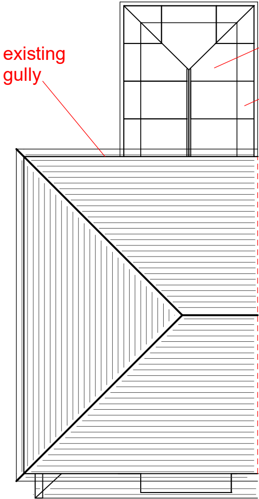
ROOF PLAN
