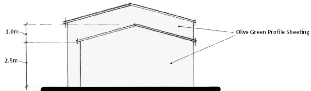
WEST ELEVATION
