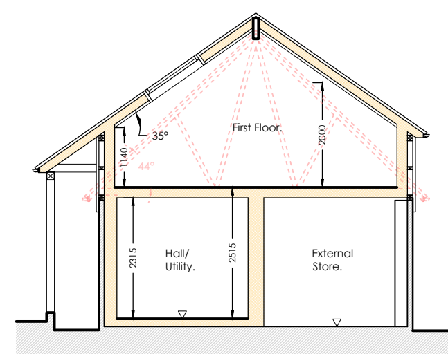
Proposed Section AA 1:100
