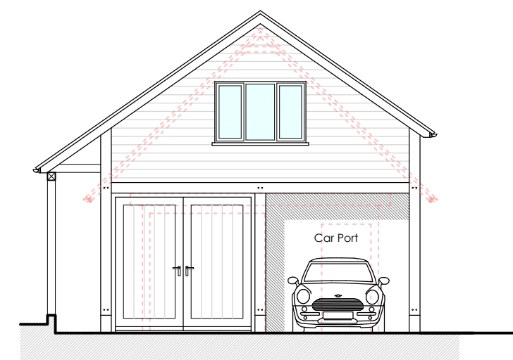
North East Elevation 1:100
