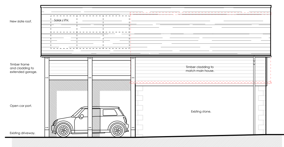
North West Elevation 1:100
