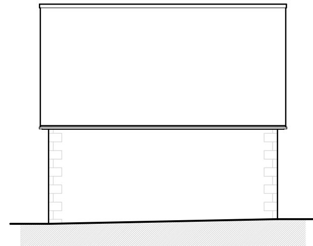
North West Elevation 1:100
