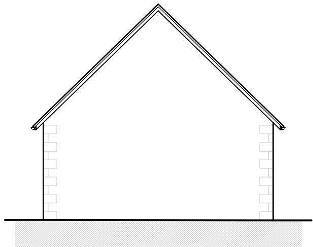
South West Elevation 1:100
