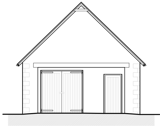
North East Elevation 1:100
