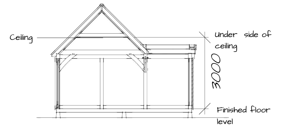
Proposed Cross-Section showing internal ceiling
