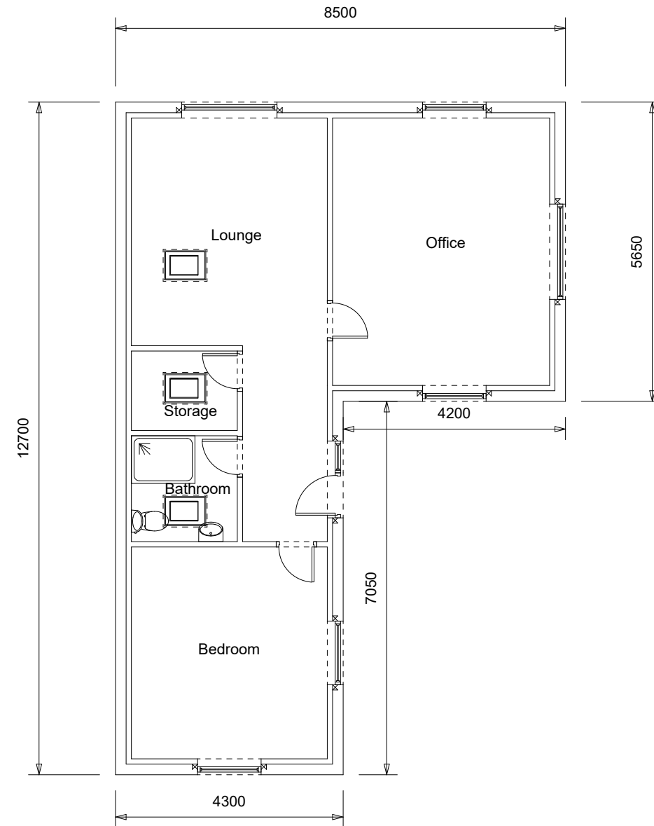
Proposed Layout
