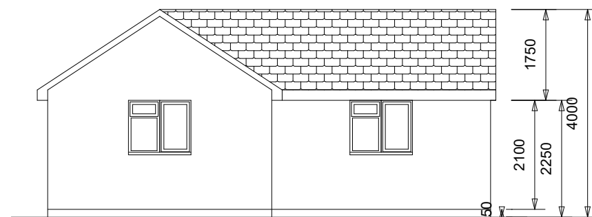
Proposed Side
