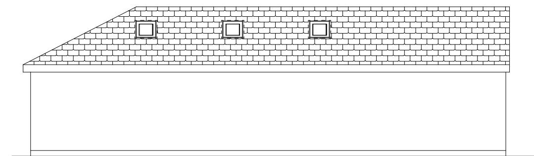
Proposed Rear
