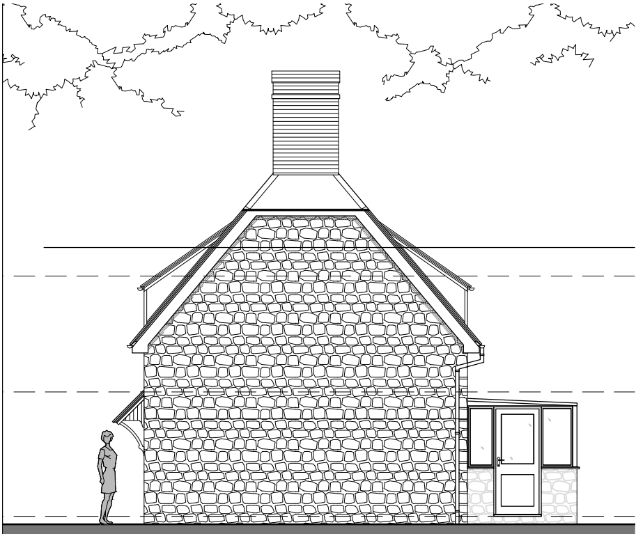
South Elevation
