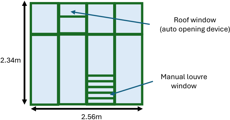
Side elevation (Facing SE, away from Bridleway)
