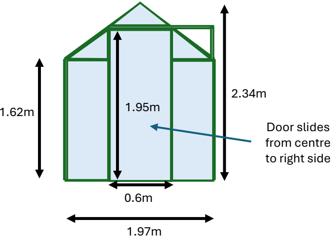
Rear elevation (Facing NE, towards property)
