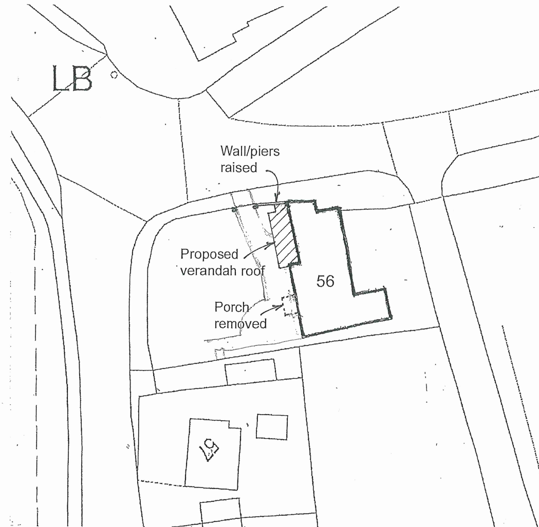
SITE BLOCK PLAN AS PROPOSED
