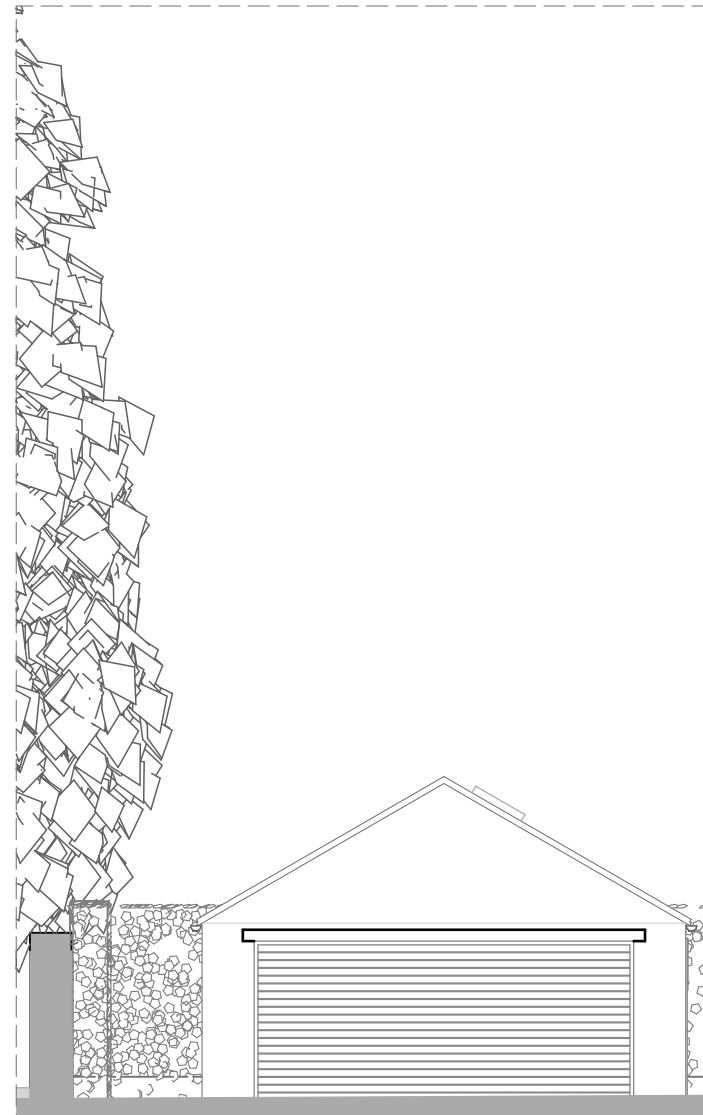
E-15 SW Elevation Proposed 1:100
