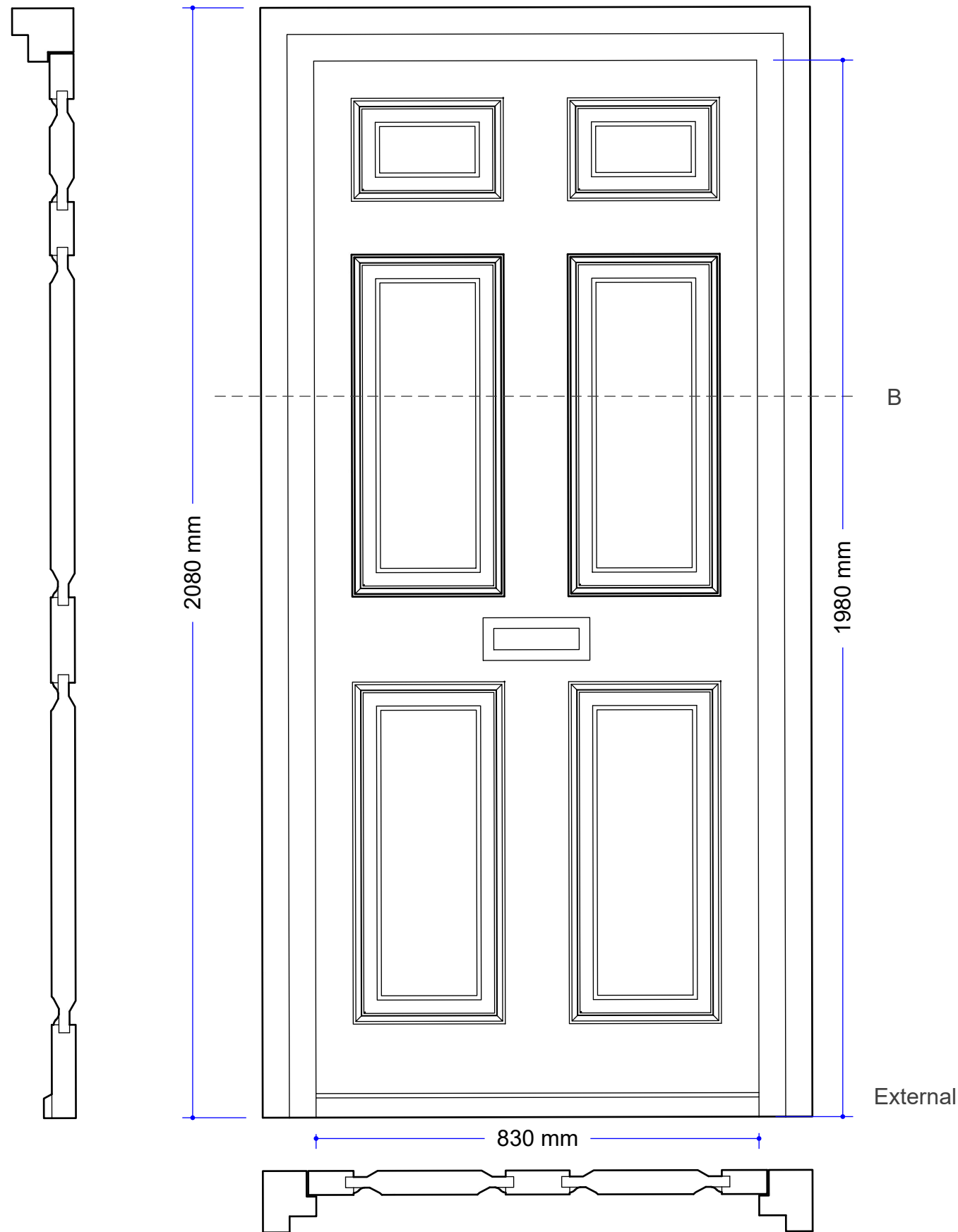
Front Door Drawings - External and Internal - Existing and Proposed
