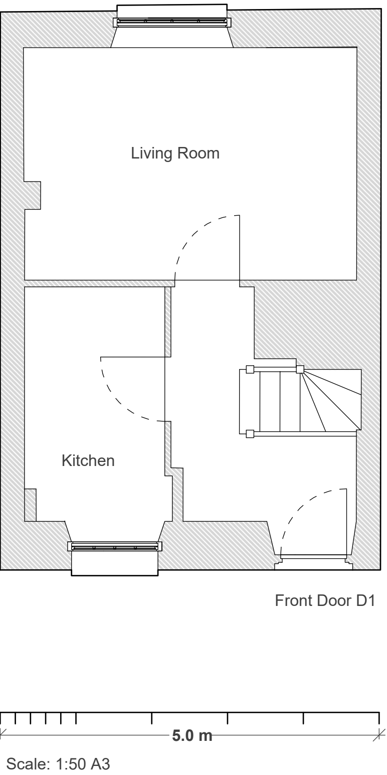
Floorplan
