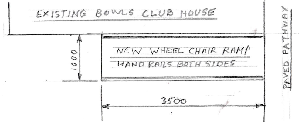
PLAN VIEW OF NEW WHEEL CHAIR RAMP
