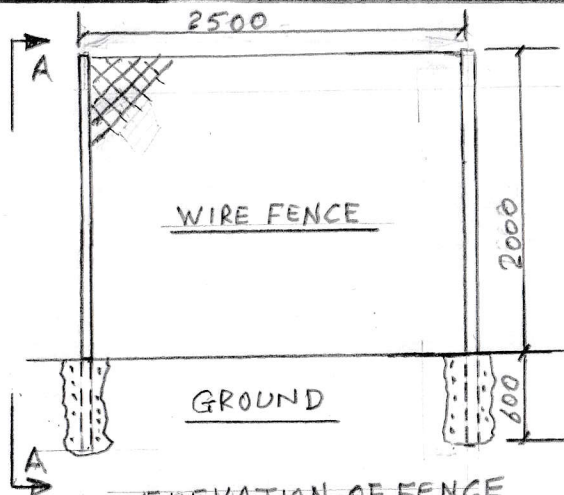
ELEVATION OF FENCE
