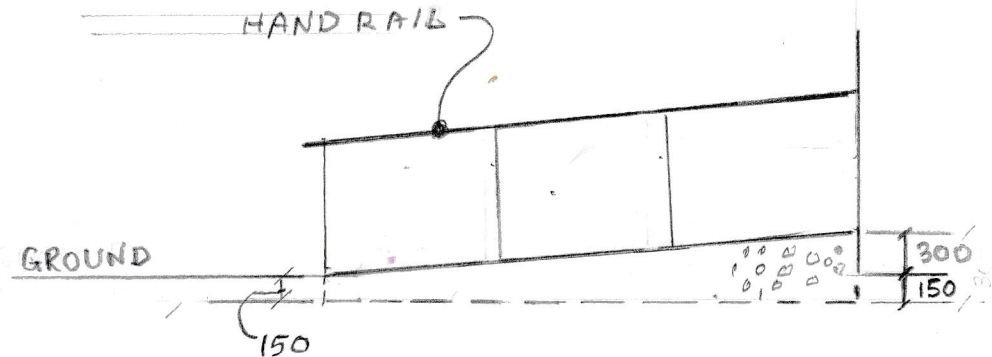
ELEVATION OF NEW WHEEL CHAIR RAMP
