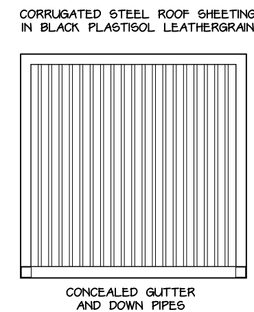
ROOF PLAN 1:50
