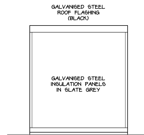
REAR ELEVATION 1:50
