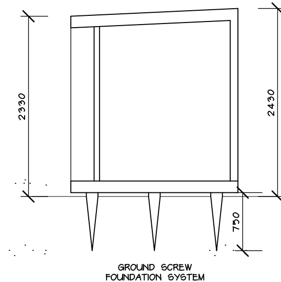
SECTION 1:50
