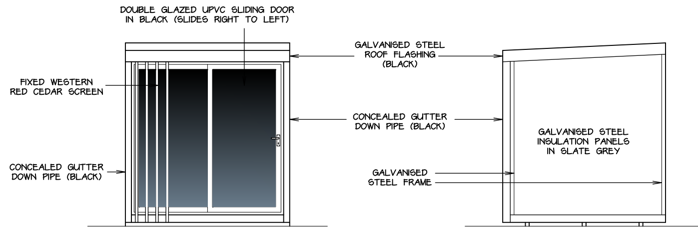
FRONT ELEVATION 1:50
