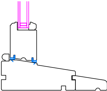
Bottom Rail
