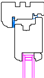
Door Head Rail
