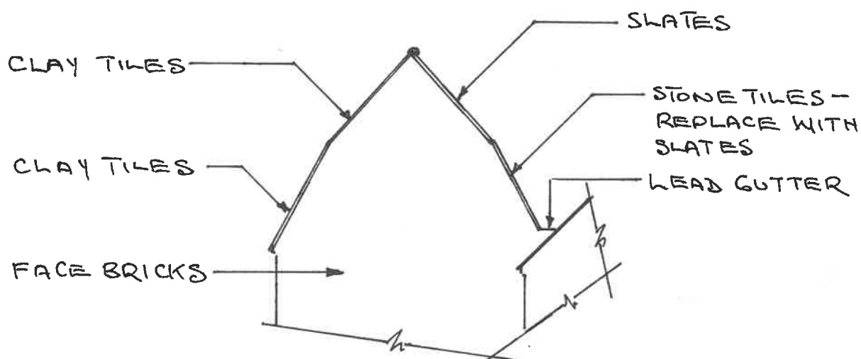
NORTH ELEVATION
