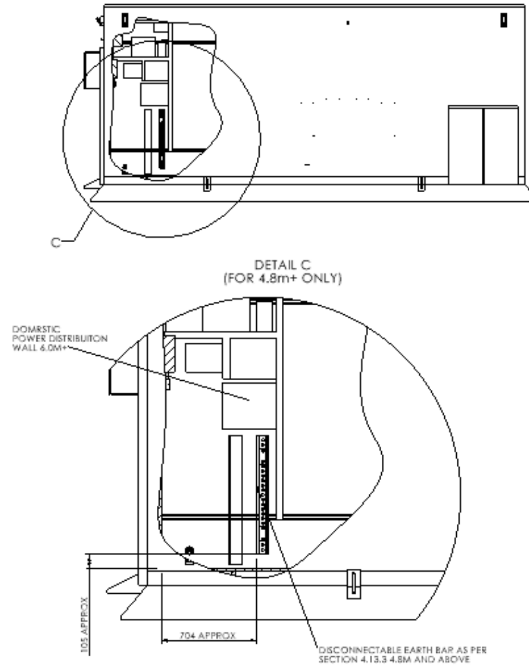
DETAIL OF 12-WAY EARTH BAR FOR BUILDINGS 4.8M AND ABOVE
