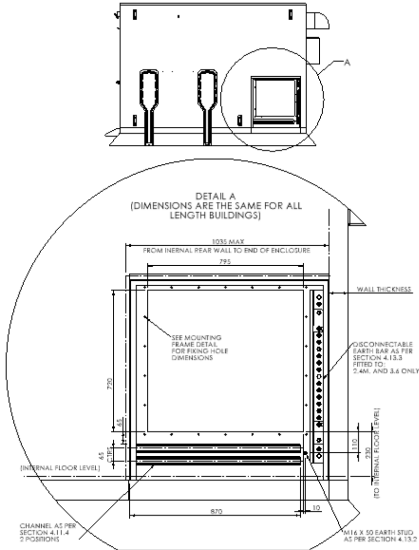
DETAIL OF LOWER SIDE ENCLOSURE (SEE SECTION 4.9.6) DIMENSIONS ARE COMON TO ALL BUILDING LENGTHS
