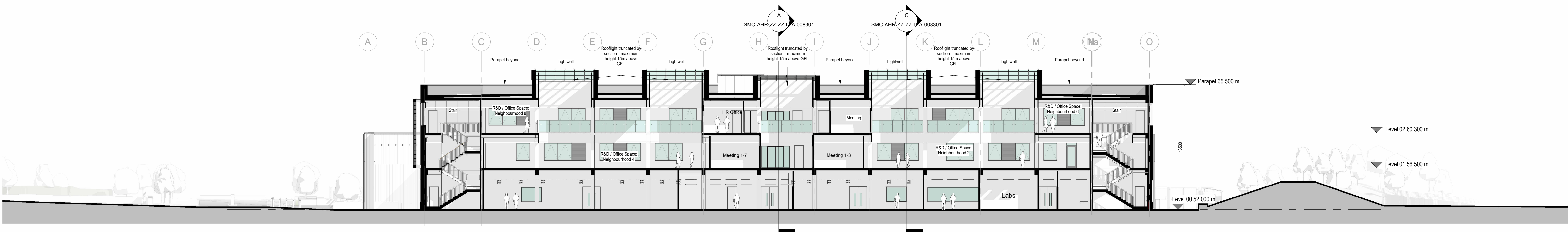
Cross Section B-B through Labs & Offices 1 : 200
