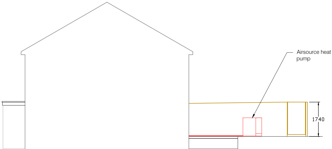
East Elevation
