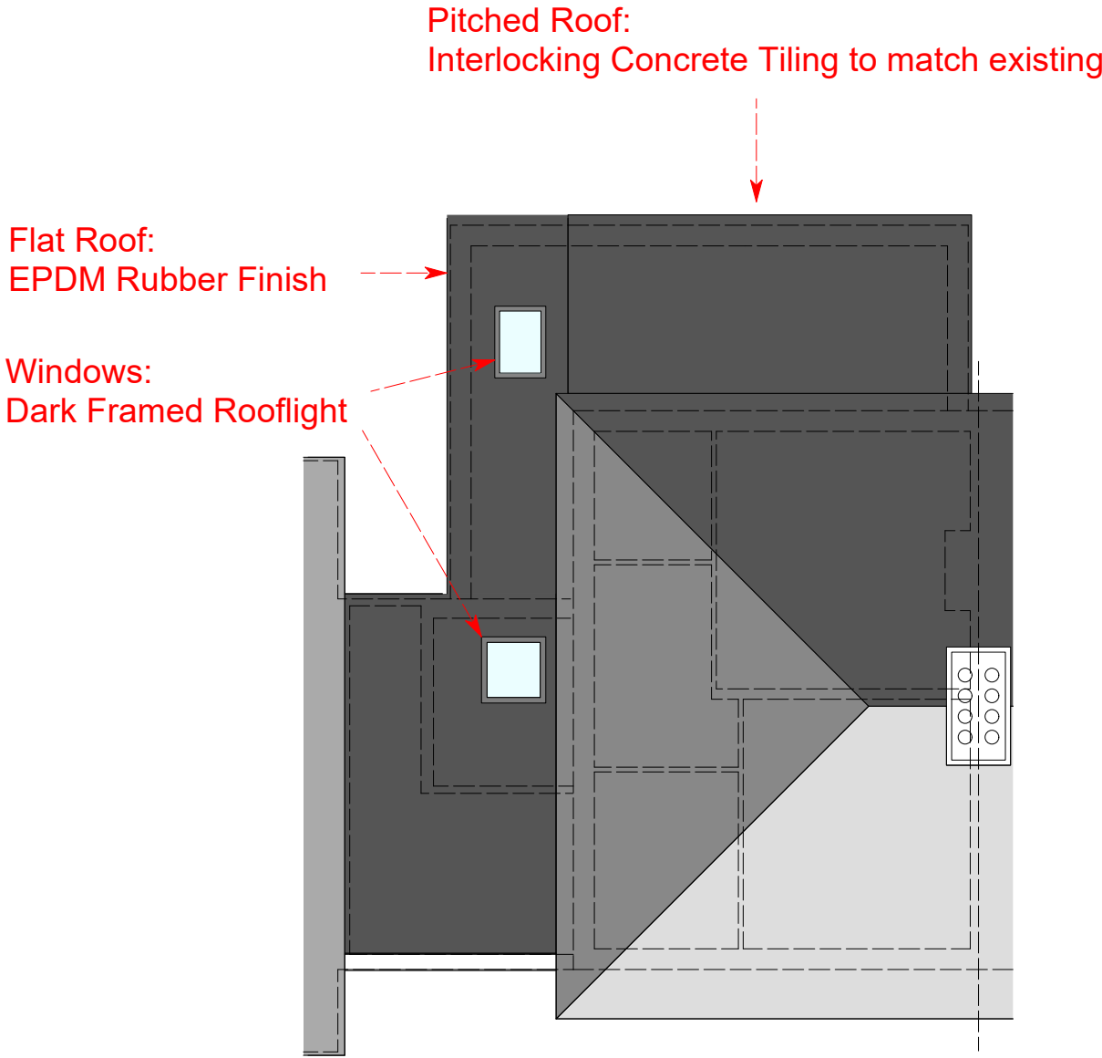
PLN 03 Proposed Roof Plan 1:100
