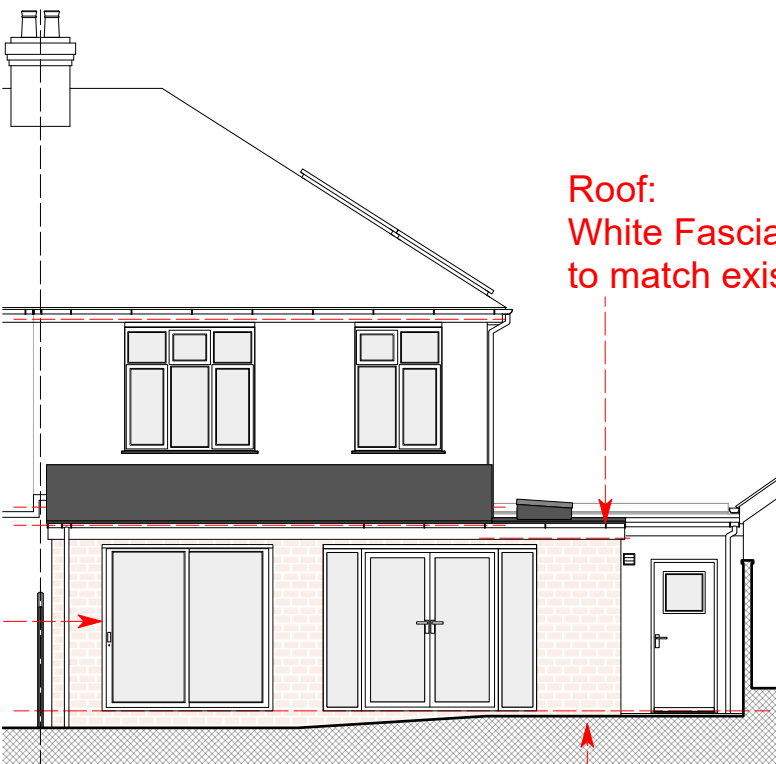
ELV 03 Proposed N Elevation 1:100
