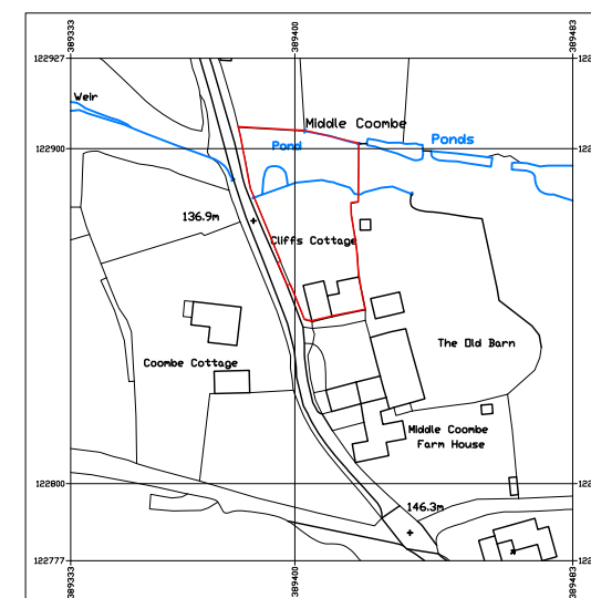
LOCATION PLAN 1:2500
