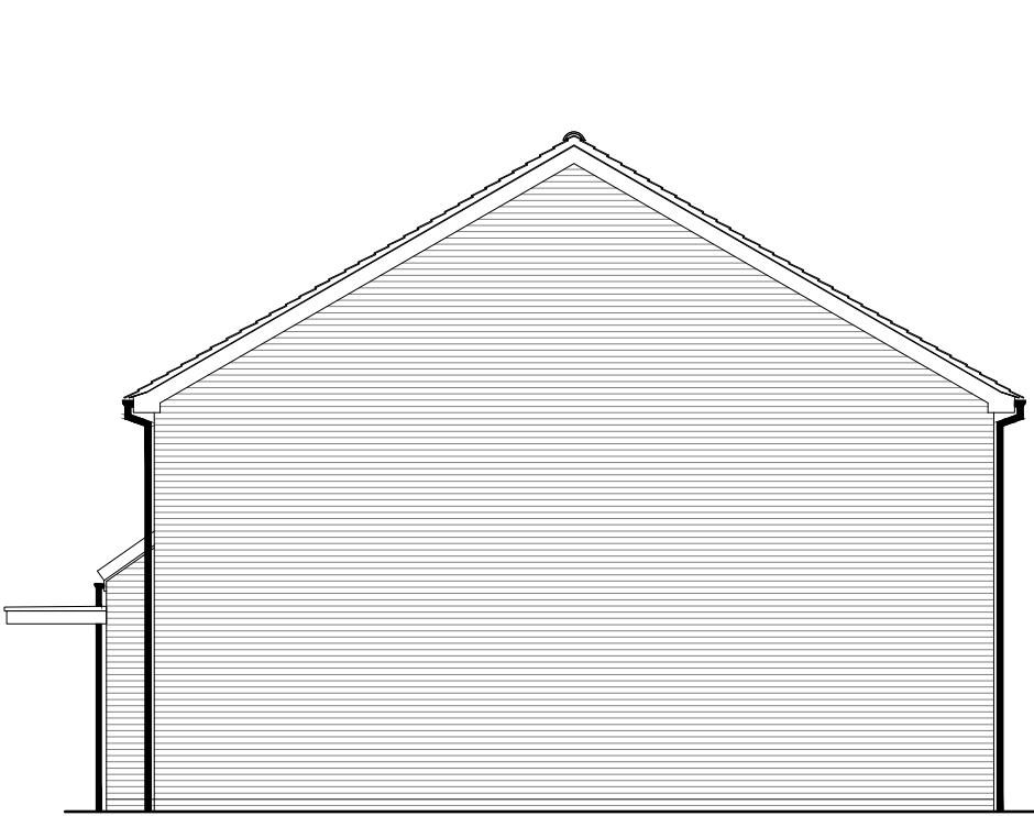
Left Elevation
