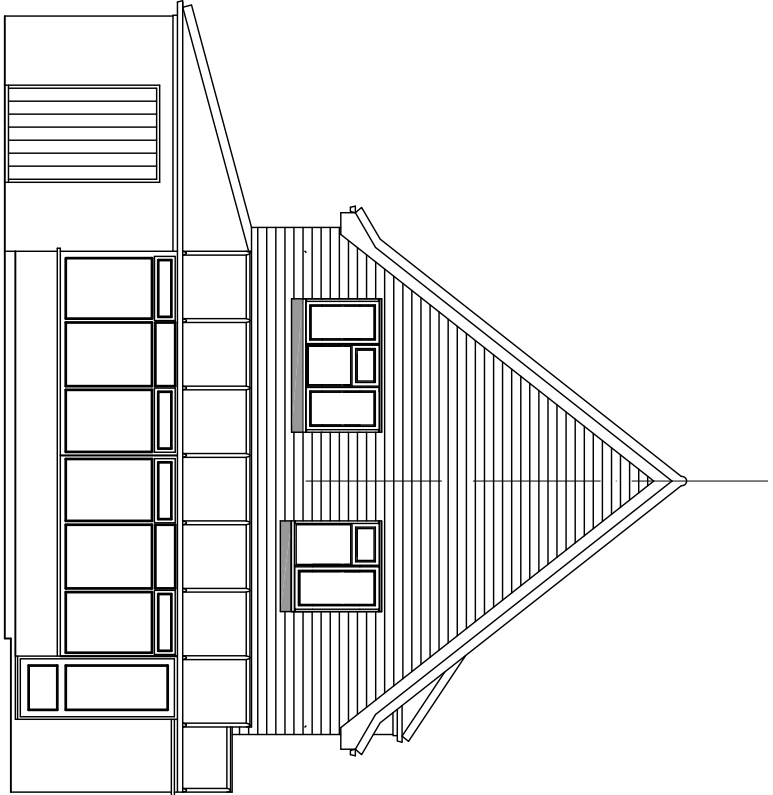
EAST ELEVATION
