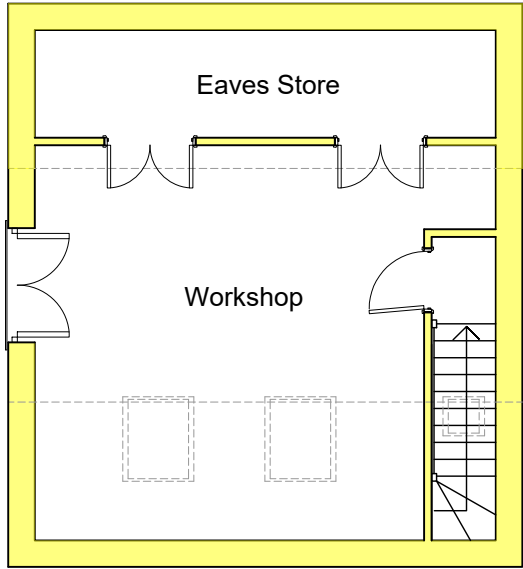
Proposed First Floor Plan - 1:100
