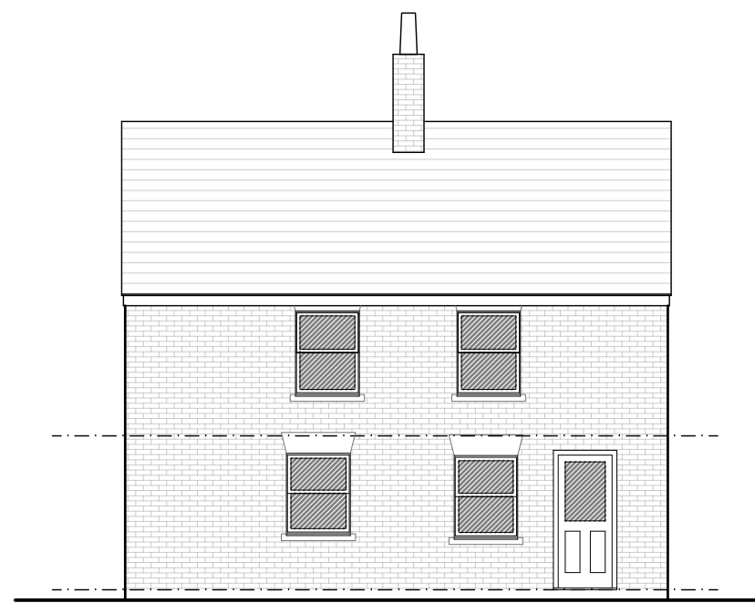
Existing South Elevation - 1:100
