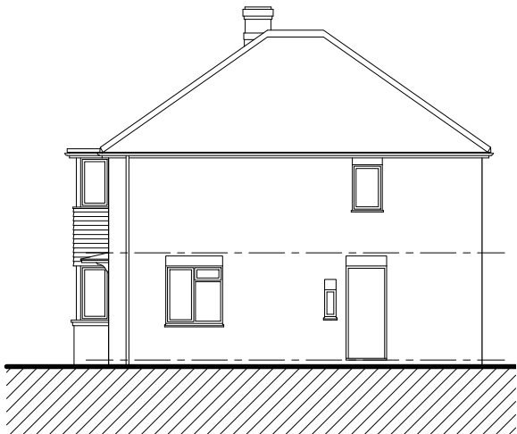
East Elevation
