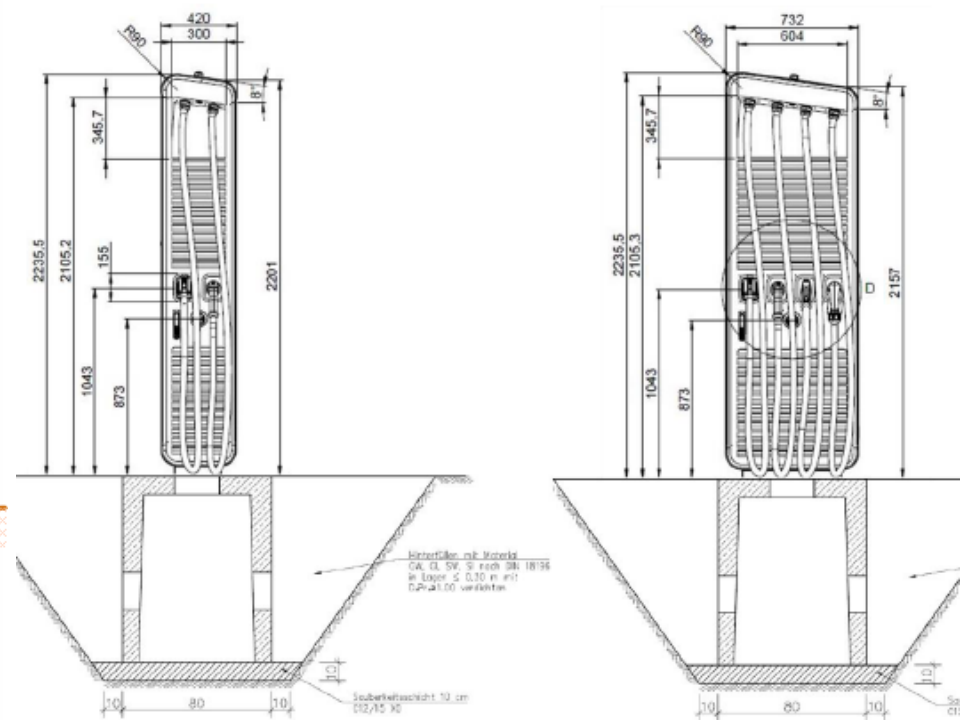
Image 2: Front view of HYC-150 and HYC-300
