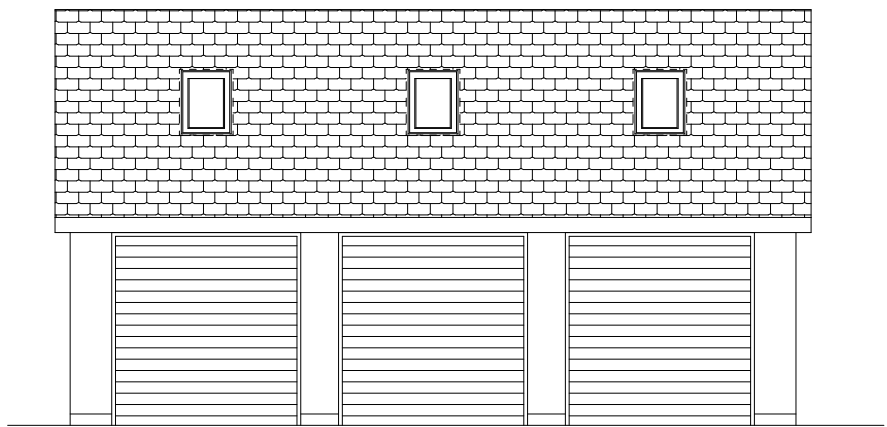
Proposed Front
