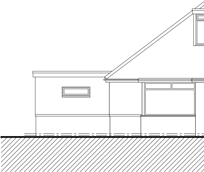
East Elevation
