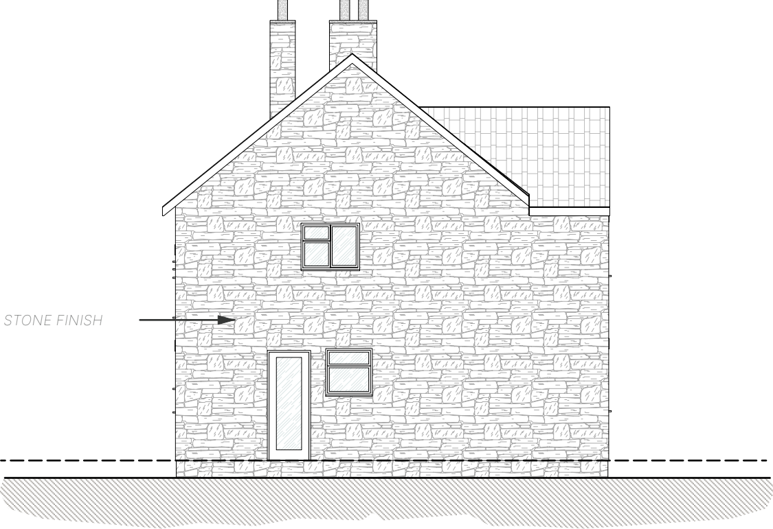
SIDE ELEVATION
