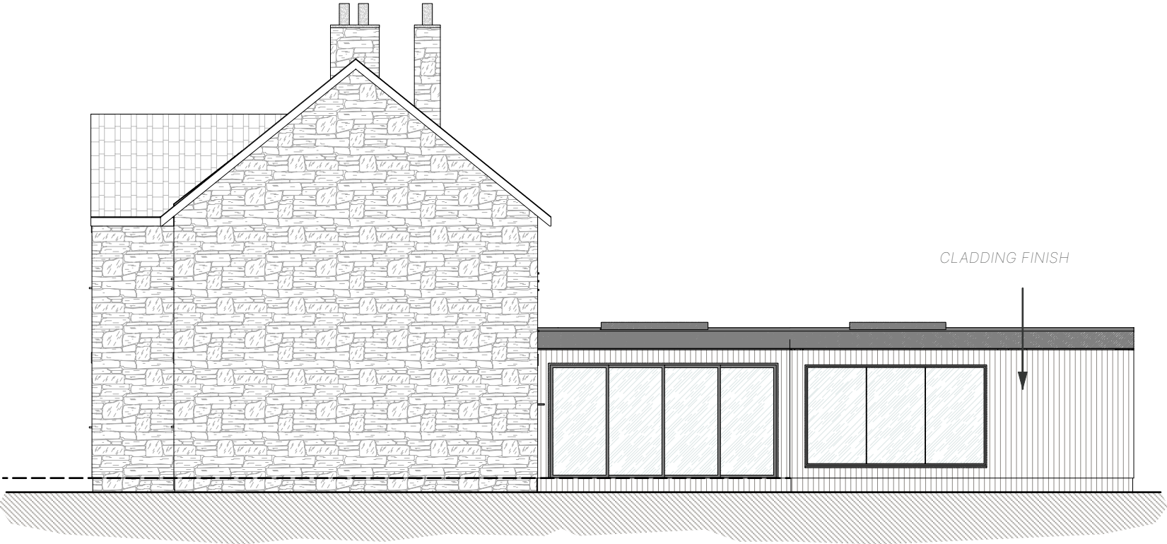
SIDE ELEVATION
