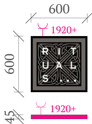
Drawing of lightbox logo
