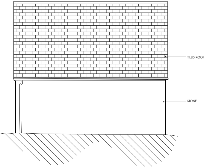
PROPOSED WEST ELEVATION 1:100
