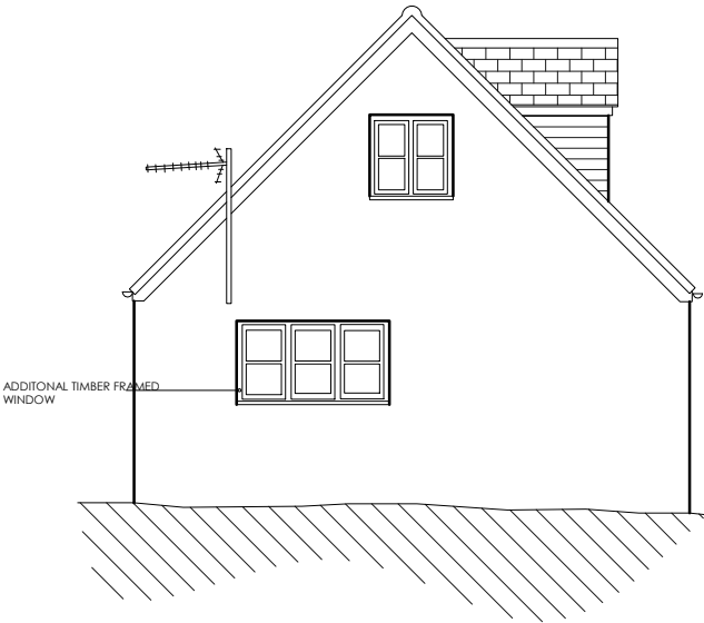
PROPOSED SOUTH ELEVATION 1:100
