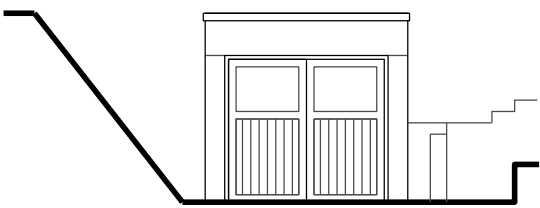
FRONT ELEVATION 1:100
