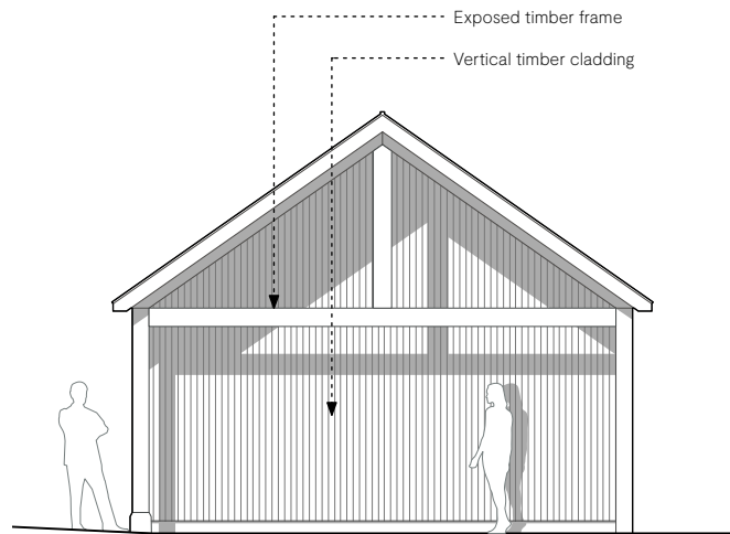
South Elevation
