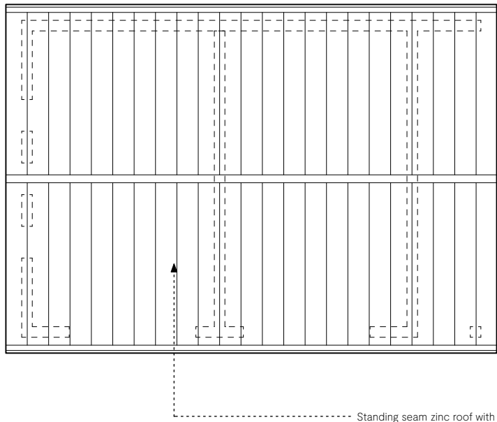
Roof Plan
