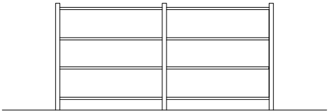
1m High 4 Bar Metal Railings (Railings & all fixtures & fittings Painted Black)
