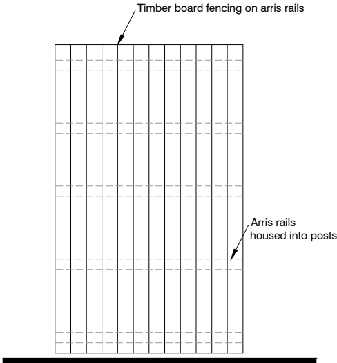
3m High Timber Acoustic Fence
