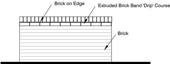
1m High Bin Screen Wall
