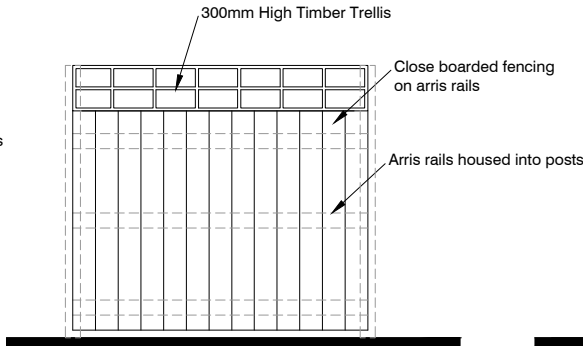
1.5m High Close Board Fence with 300mm Timber Trellis
