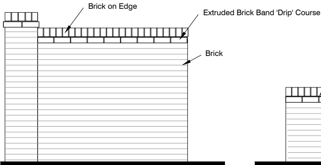
1.8m High Brick Screen Wall 2m High Brick Piers where shown
