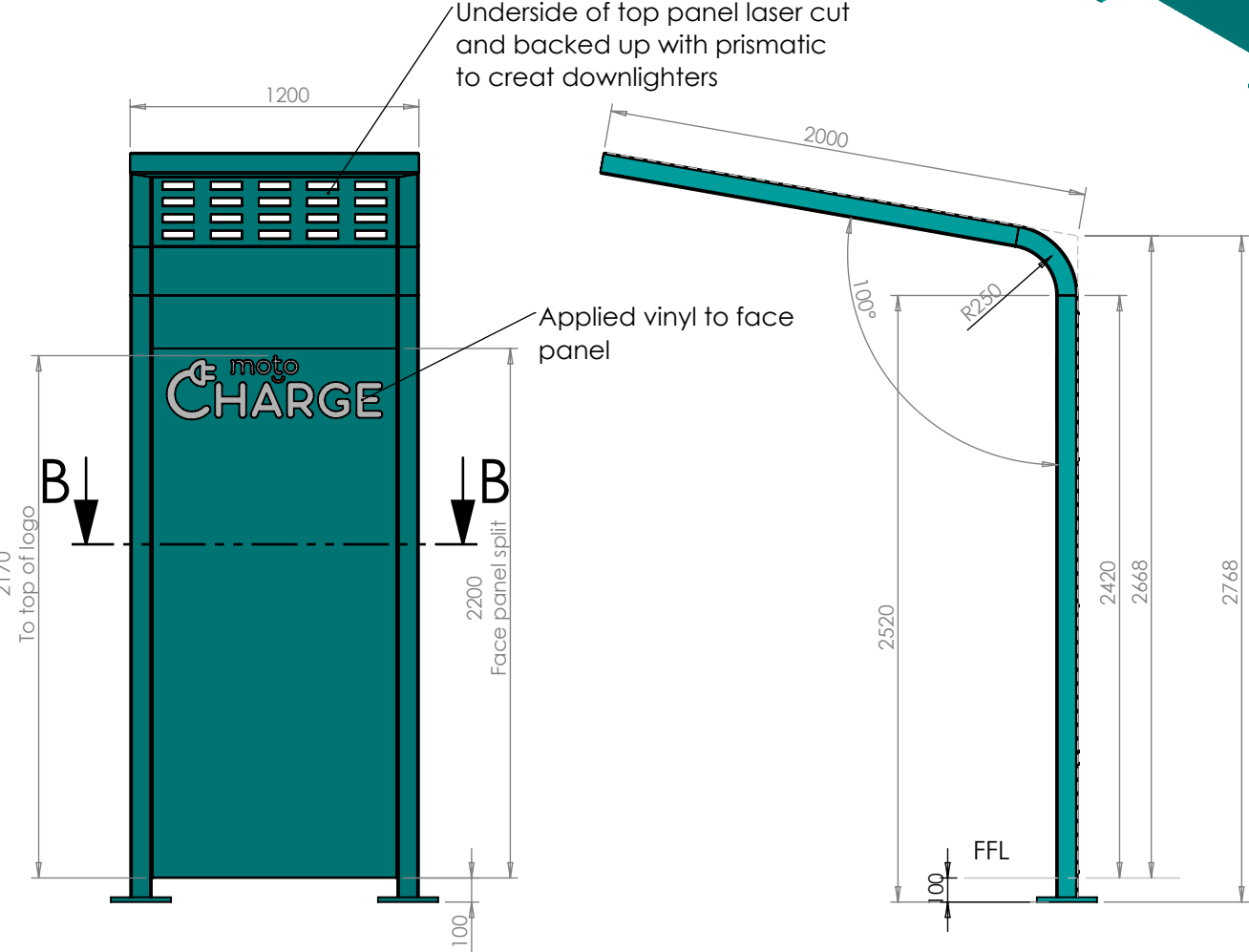
Front view
