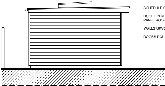
NORTH WEST ELEVATION OF NEW GARDEN ROOM
