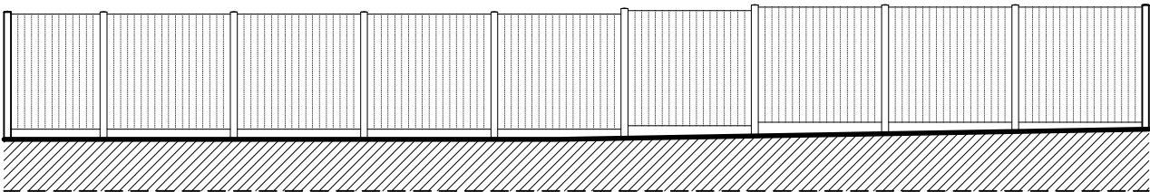
INTERNAL GARDEN ELEVATION OF REPLACED FENCE
