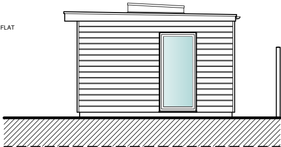
SOUTH EAST ELEVATION OF NEW GARDEN ROOM
