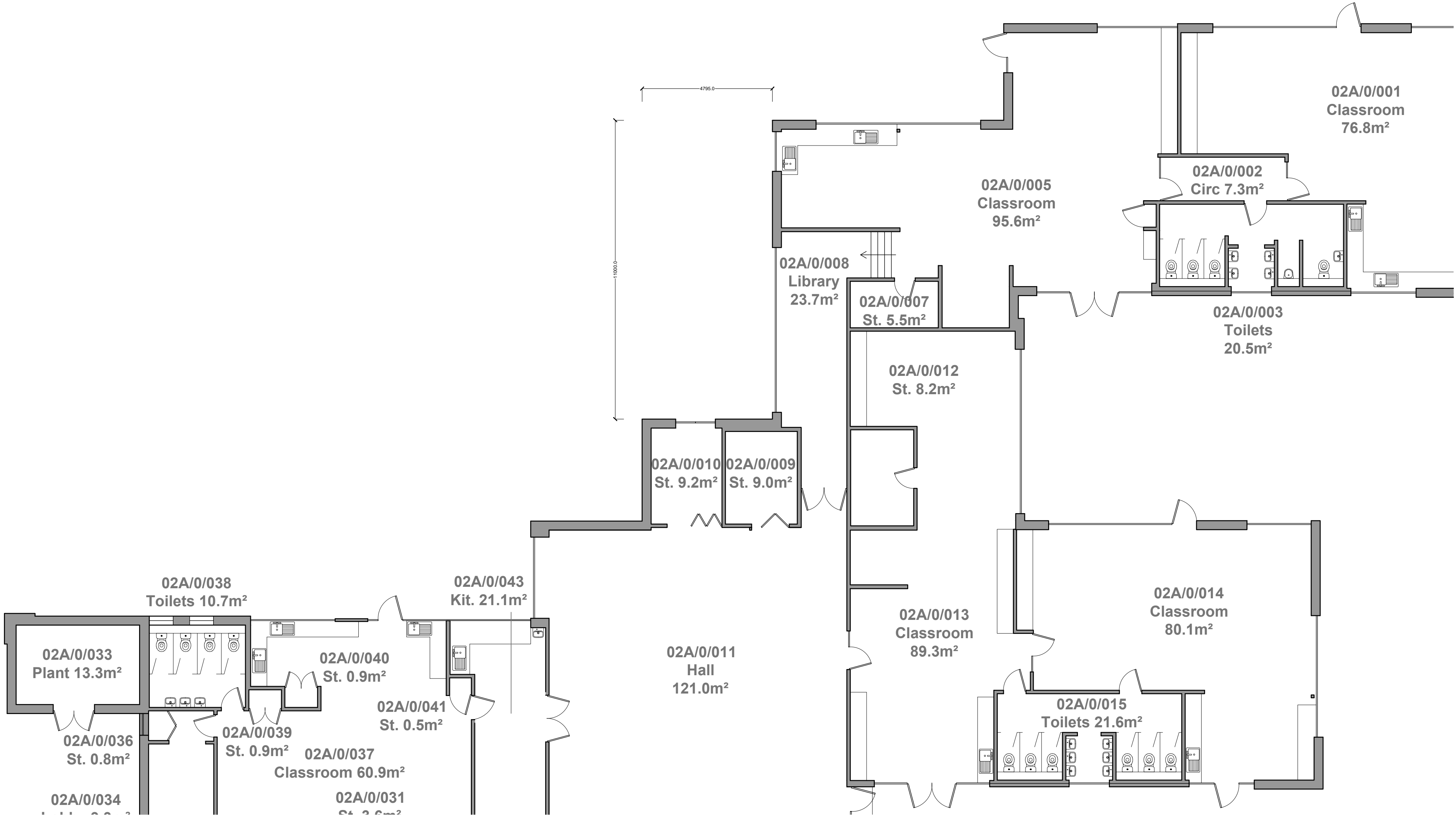
Existing Layout Scale 1:100 @ A2
