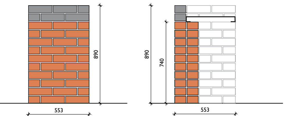
Side Elevation:
