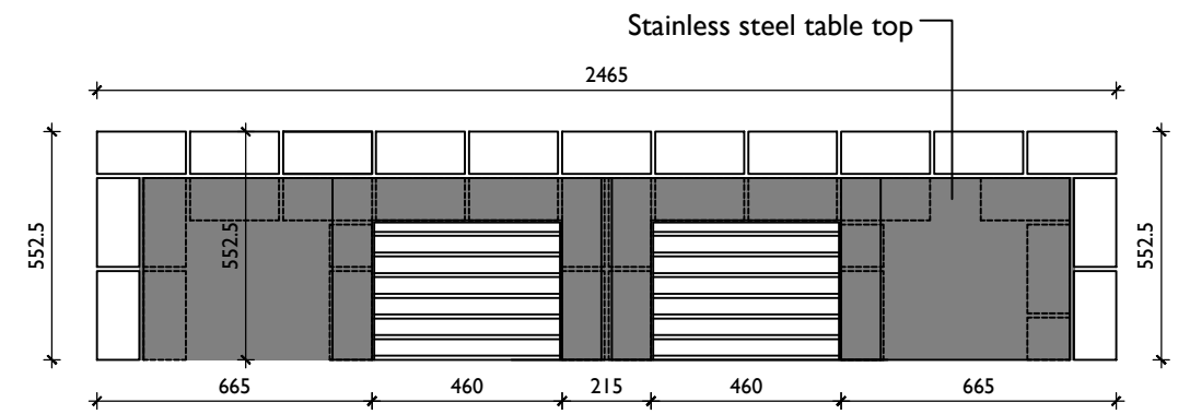
4 Bed Exec/ Exclusive & 6 Bed Woodland- Plan:
