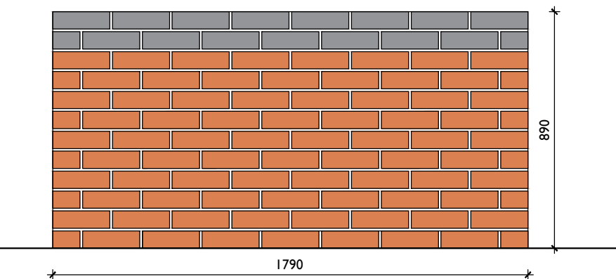
Rear Elevation:
