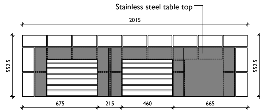
4 Bed Woodland- Plan:
