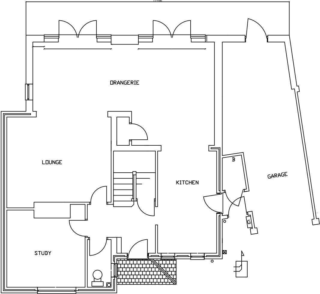
Ground Floor Plan- Existing
