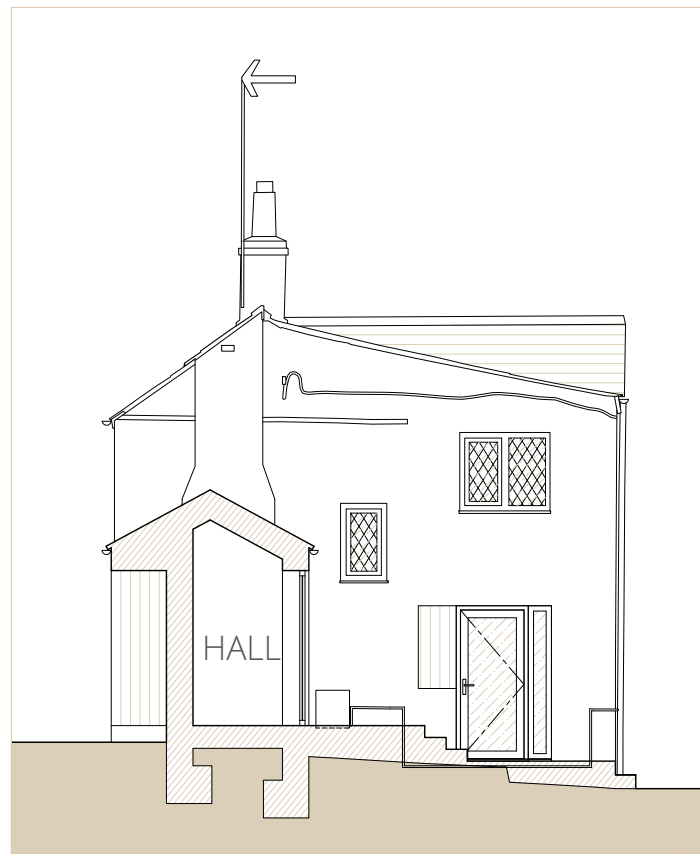
SECTION - VIEW E
